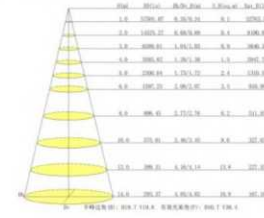
100W照度图 100W Illumination curve
