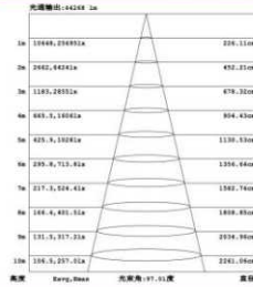
QCB-400W 90° 照度图 QCB-400W 90° Illumination curve
