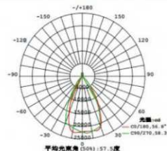
200W 60° 配光曲线 200W 60° Light distribution curve
